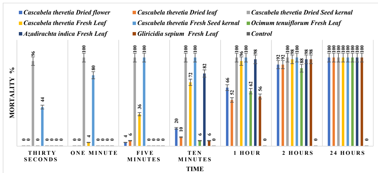
Figure 2. Mortality % of red flour beetle to different plant extracts.
