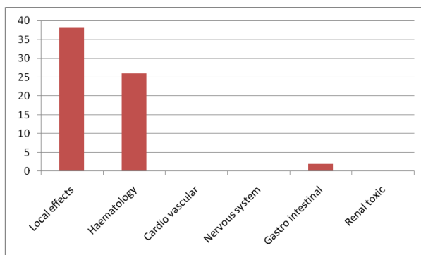
Fig. 9: Clinical profile of Saw scaled viper (38 cases)
