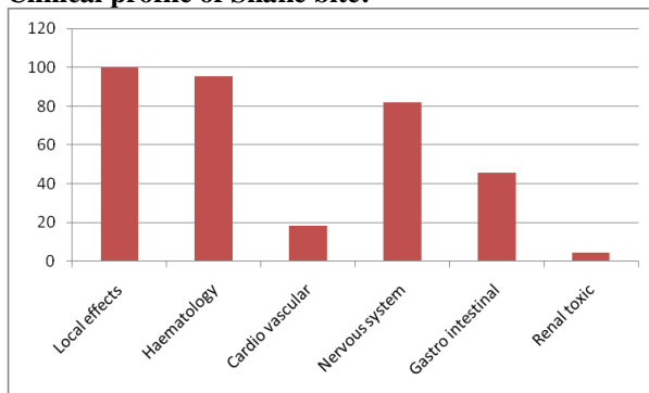
Fig. 8: Clinical profile of Russell's viper (22 cases)
