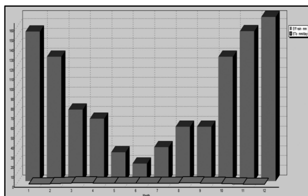
Fig 1: Effective rainfall and References Evapotranspiration
