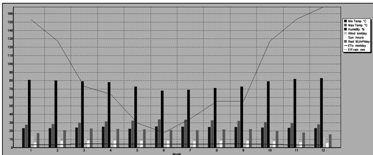
Fig 2: Climate data, reference evapotranspiration and effective rainfall
