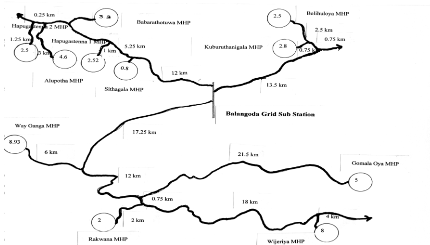
Figure 1: Mini Hydro Plants Connected to Balangoda grid Substation
