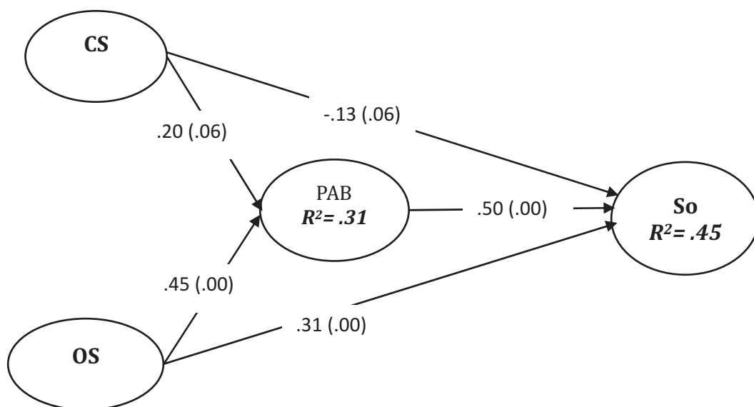
Figure 1: Path Coefficient and Its Significance
