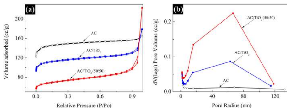
Figure 5. (a) Nitrogen adsorption–desorption isotherms and (b) BJH pore-size distributions of the AC, AC/TiO 2 (80:20), and AC/TiO 2 (50:50) films.
