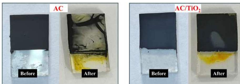
Figure 7. AC and AC/TiO 2 CEs before and after the fabrication of DSSCs.
