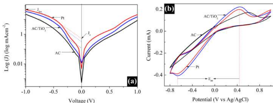
Figure 9. (a) Tafel polarization curves. (b) Cyclic voltammogram for AC/TiO 2 , AC, and Pt CEs.
