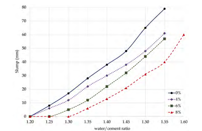
Fig 4. Variation of slump along with water/cement ratio for various mortar mix
