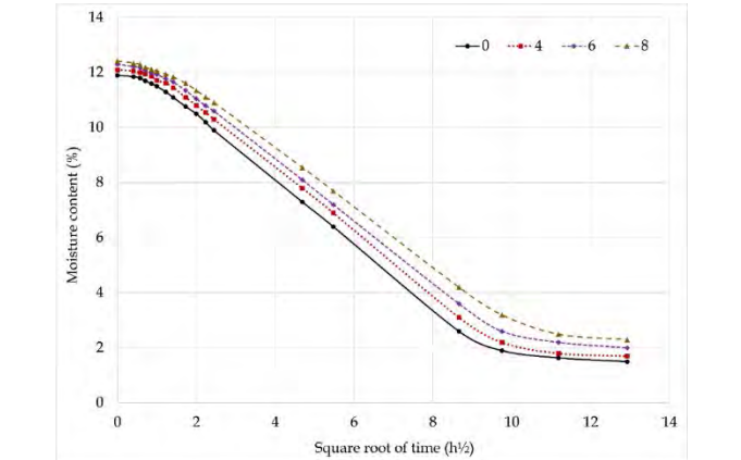
Fig 6. Moisture content variation with elapsed time
