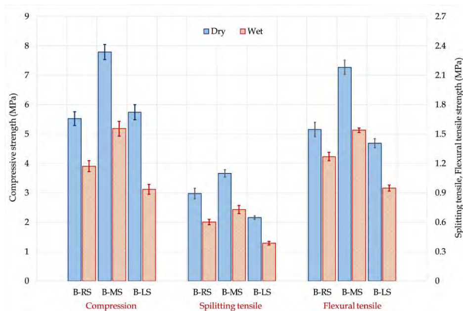
Fig. 3 - Mechanical properties of the blocks
