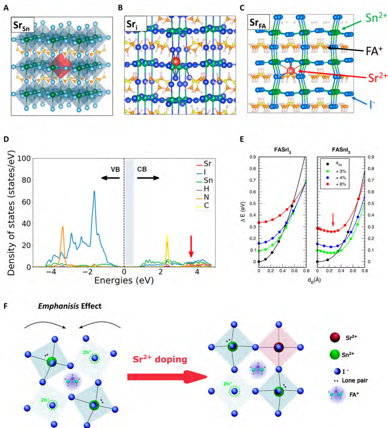
Figure 2. Interaction of \text{Sr}^{2+} in the crystal structure of FASl. A) \text{Sn}^{2+} substitution by \text{Sr}^{2+} ; B) \text{Sr}^{2+} in the interstitial position; C) \text{Sr}^{2+} substituting the \text{A}^+ cation. D) DFT-GGA atom-projected density of states (pDOS) for substitutional \text{Sr}_{\text{Sn}} . E) Energy landscape for cation off-centering displacement in \text{FASrI}_3 and \text{FASrIn}_3 at various expanded lattice parameter a . F) Proposed healing mechanism of the tilting and tin off-centering upon \text{Sr}^{2+} doping.
