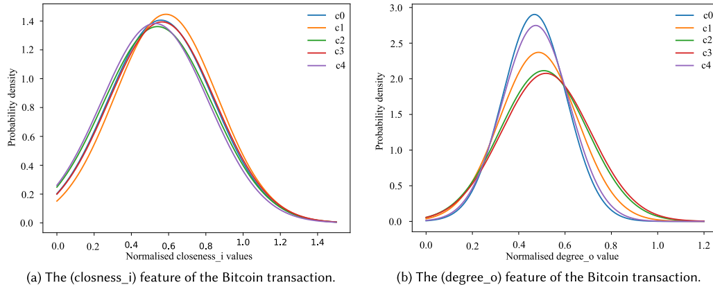
Fig. 4. Probability distribution of the closeness_i and degree_o features in the AP -based clusters.
