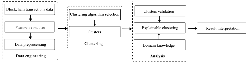
Fig. 1. Overview of the proposed methodology.
