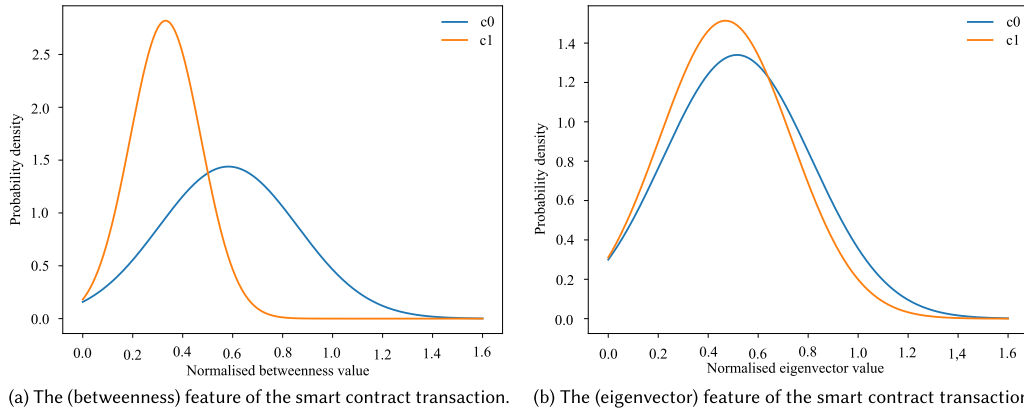
Fig. 7. Probability distribution of the betweenness and eigenvector features in the Spectral -based clusters.
