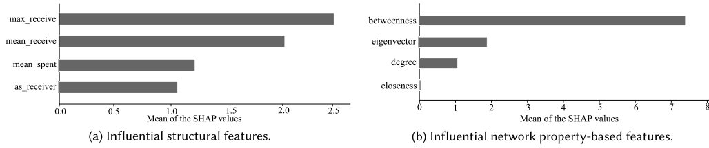
Fig. 5. SHAP values for the features of Ethereum Ponzi contract transactions based on spectral clustering outcomes.
