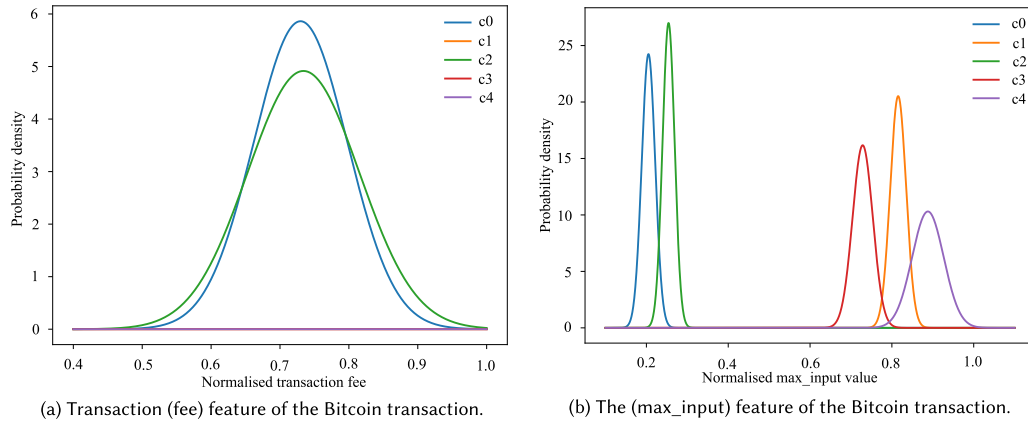
Fig. 3. Probability distribution of the transaction fee and max_input features in the AP -based clusters.
