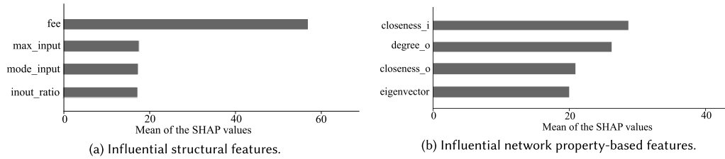
Fig. 2. SHAP values for the features of Bitcoin ransomware transactions based on AP outcomes.
