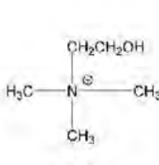
Choline
