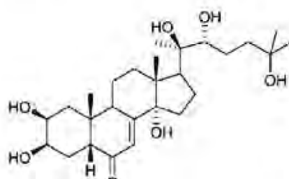
20-hydroxyecdysone
