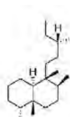
ent-neo-clerodane
