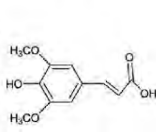
Sinapic acid
