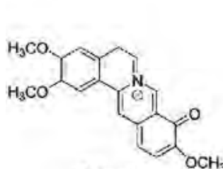
Palmatine
